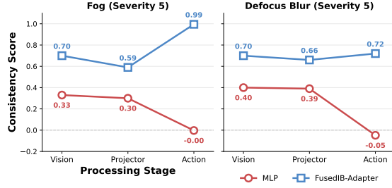
Figure 2. Feature consistency across VLA processing stages under visual corruptions (severity 5). The MLP projector shows progressive degradation from Vision to Action, with action predictions collapsing to near-random outputs. Fused IB-Adapter maintains stable representations throughout the pipeline.
