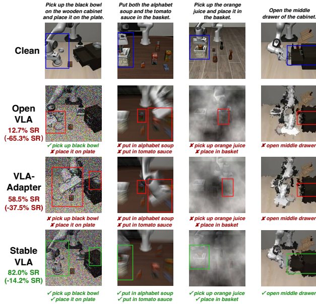
Figure 3. Cases of catastrophic failure. We evaluate baseline models and StableVLA over noise, blur, weather and digital corruptions at level 5 corruption. While baselines such as OpenVLA and VLA-Adapter exhibit significant performance degradation on corrupted inputs, StableVLA maintains robust performance.
