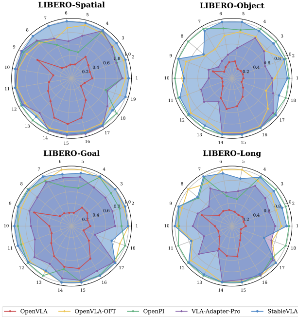
Figure 5. Robustness comparison across visual corruption types on LIBERO. Each axis represents a corruption type. See Appendix D for details.
