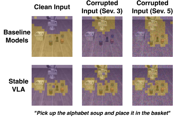
Figure 6. Semantic grouping of Fused IB-Adapter output features. We injected speckle noise at severity levels 3 and 5 into the input image of a LIBERO-Object task (“Pick up the alphabet soup and place it in the basket”). Then, we applied K-means clustering ( K=2 ) to visualize and compare the semantic clusters in the output features across clean, level-3 and level-5 noisy inputs. The comparison between baseline models and Stable VLA demonstrates that StableVLA maintains more consistent and accurate semantic grouping even under high levels of noise corruption.
