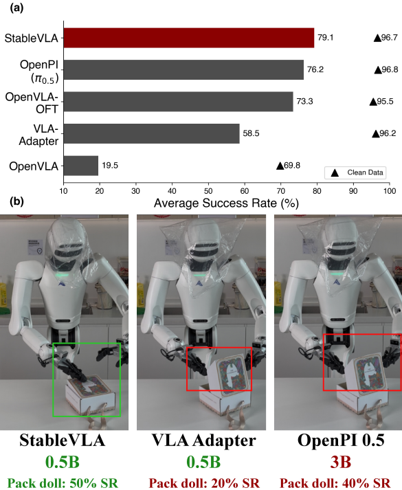
Figure 1. (a) Robustness comparison of StableVLA and other baselines. Triangle marks and bar charts denote performance on clean data and corrupted data (averaged across severities), respectively. StableVLA achieves state-of-the-art zero-shot robustness. (b) Real-world robot deployment on the Pack Doll task under visual corruptions. StableVLA (0.5B) achieves 50% success rate, outperforming both VLA-Adapter (0.5B, 20%) and OpenPI 0.5 (3B, 40%) despite having fewer parameters.
