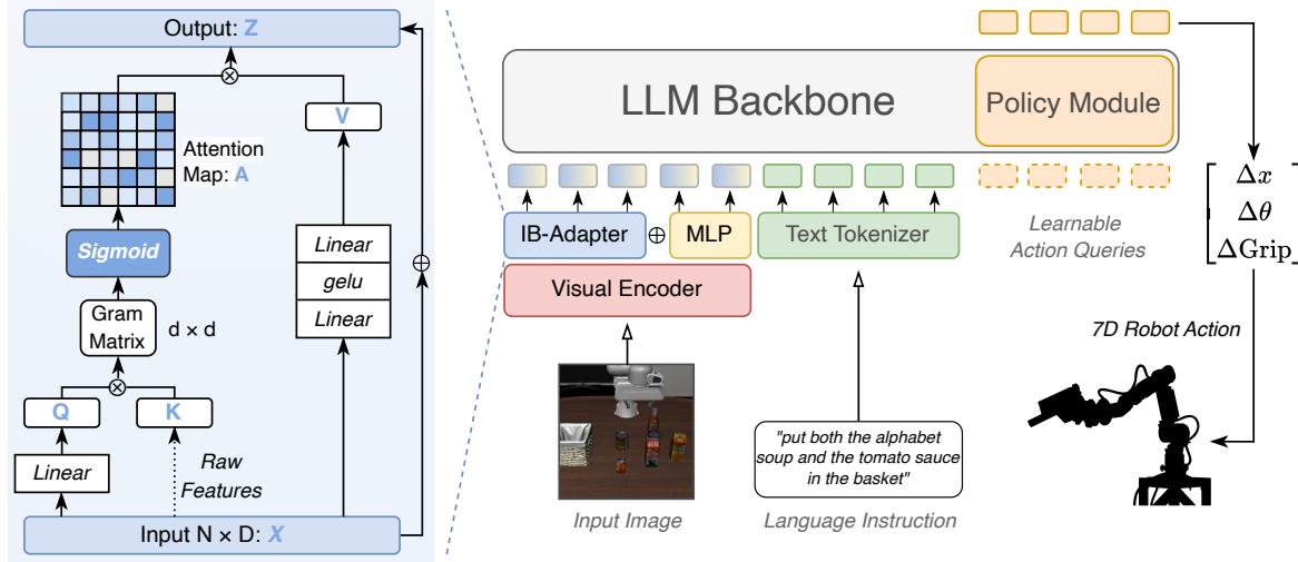
Figure 4. Architecture of the IB-Adapter and StableVLA. We replace the standard linear bottleneck in StableVLA with Fused IB-Adapter. IB-Adapter processes visual tokens \mathbf{X} via three parallel pathways to enforce subspace filtering: (1) Covariance Attention: We utilize raw features as keys (dotted line) to preserve original geometric structure. We compute the Gram Matrix ( D \times D ) to capture global channel correlations. (2) Sigmoid Gating: A learnable Sigmoid function generates the Attention Map \mathbf{A} , acting as an independent gate to suppress noise. (3) Feature transformation: Features undergo non-linear transformation before reconstruction.
