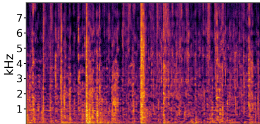
SCORE-CLAP
