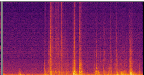
SCORE-TILT
