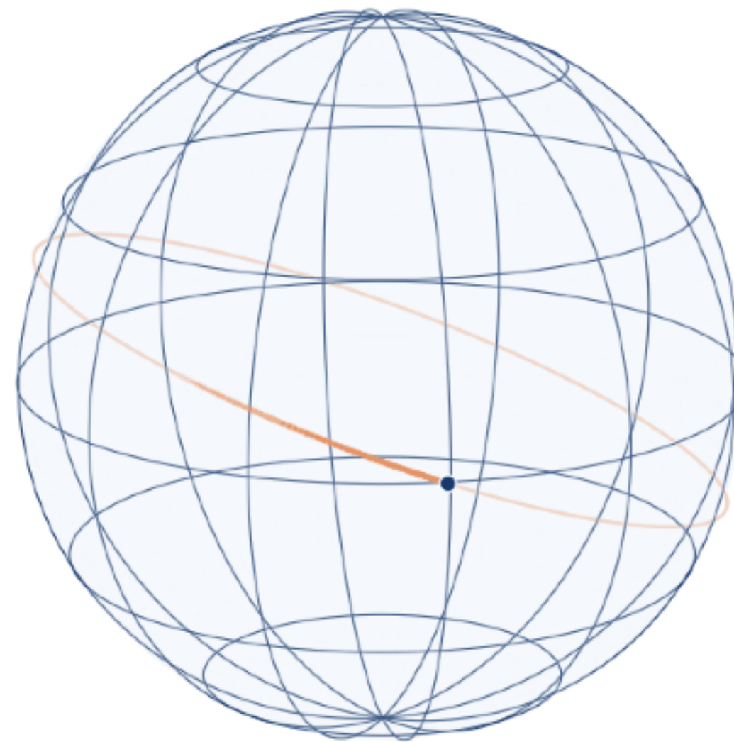
a sphere
