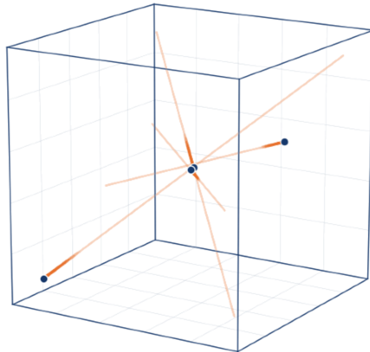
flat space
