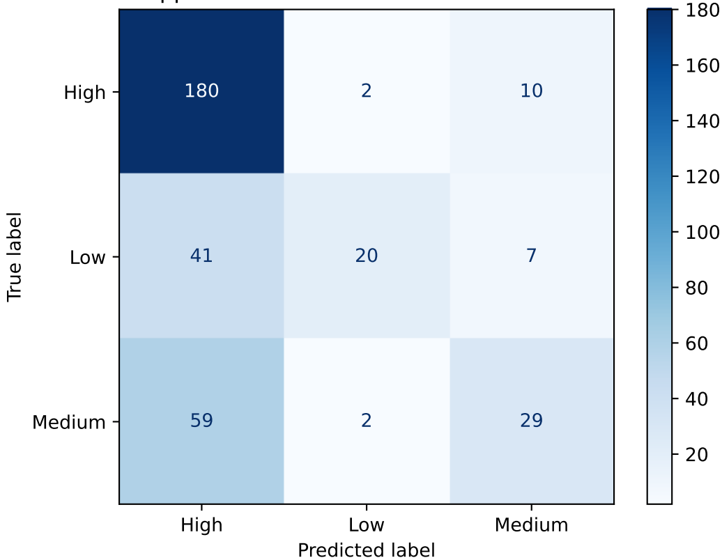
Support Vector Classifier Confusion Matrix
