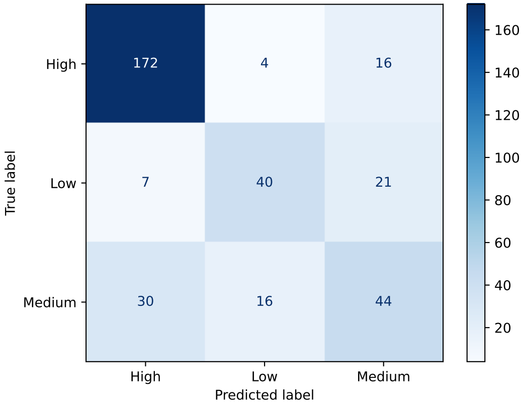
TabPFNClassifier Confusion Matrix
