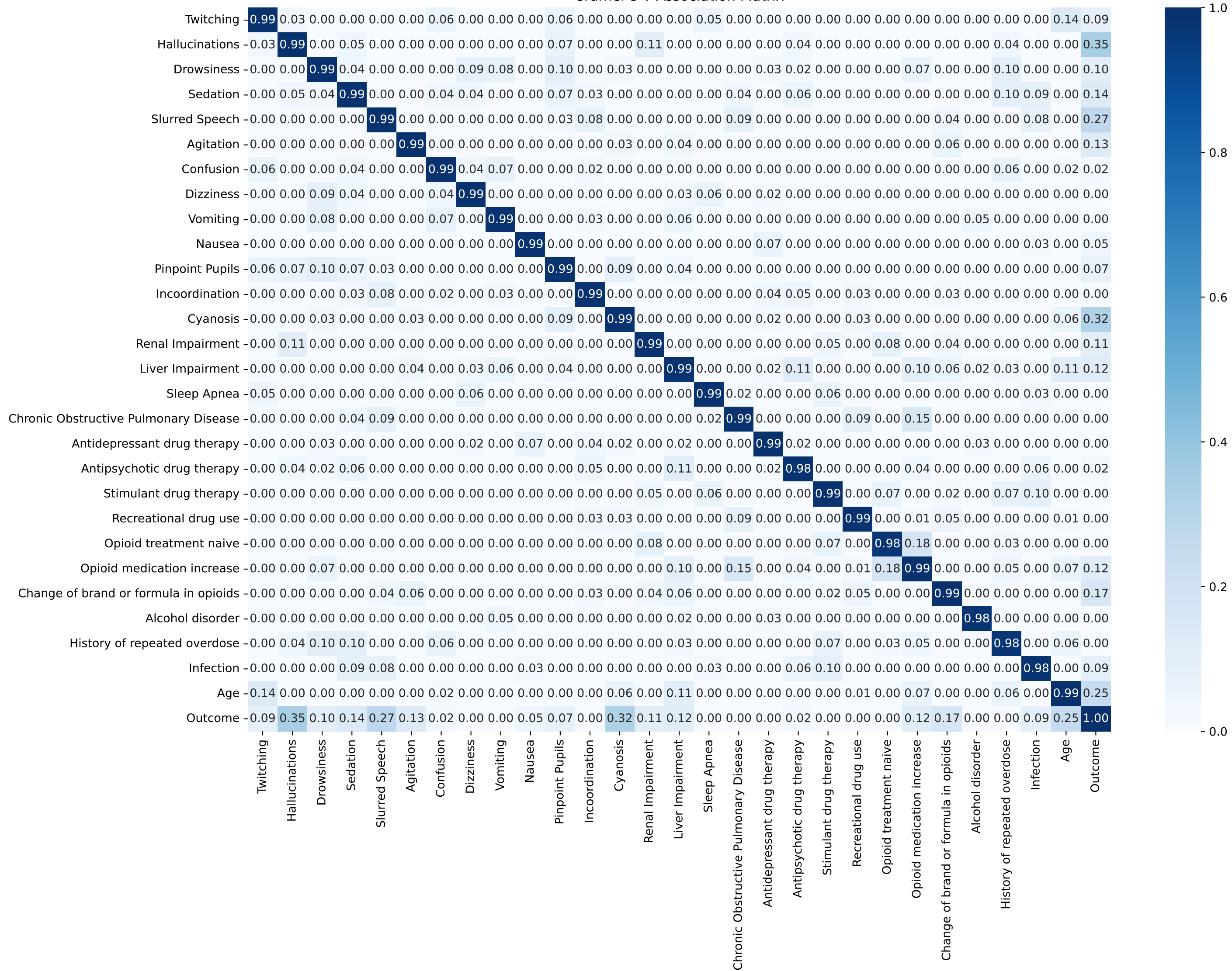
Cramér's V Association Matrix
