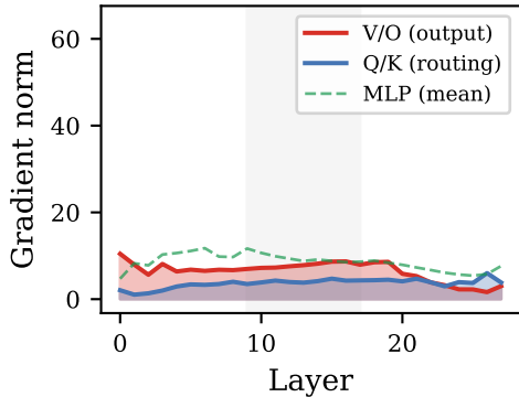
Qwen2.5-7B V/O:Q/K = 1.76×
