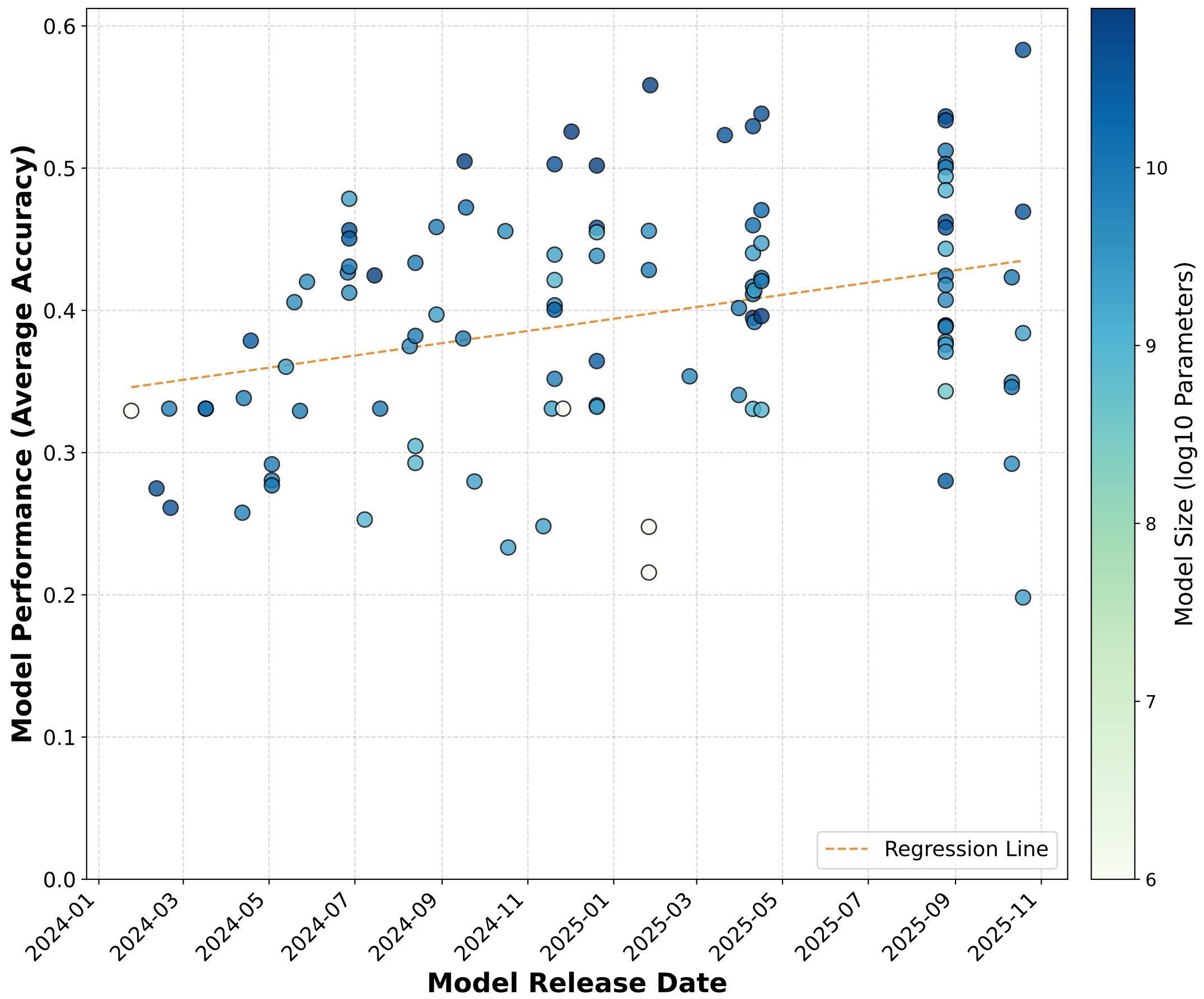
Model Performance vs Release Date
