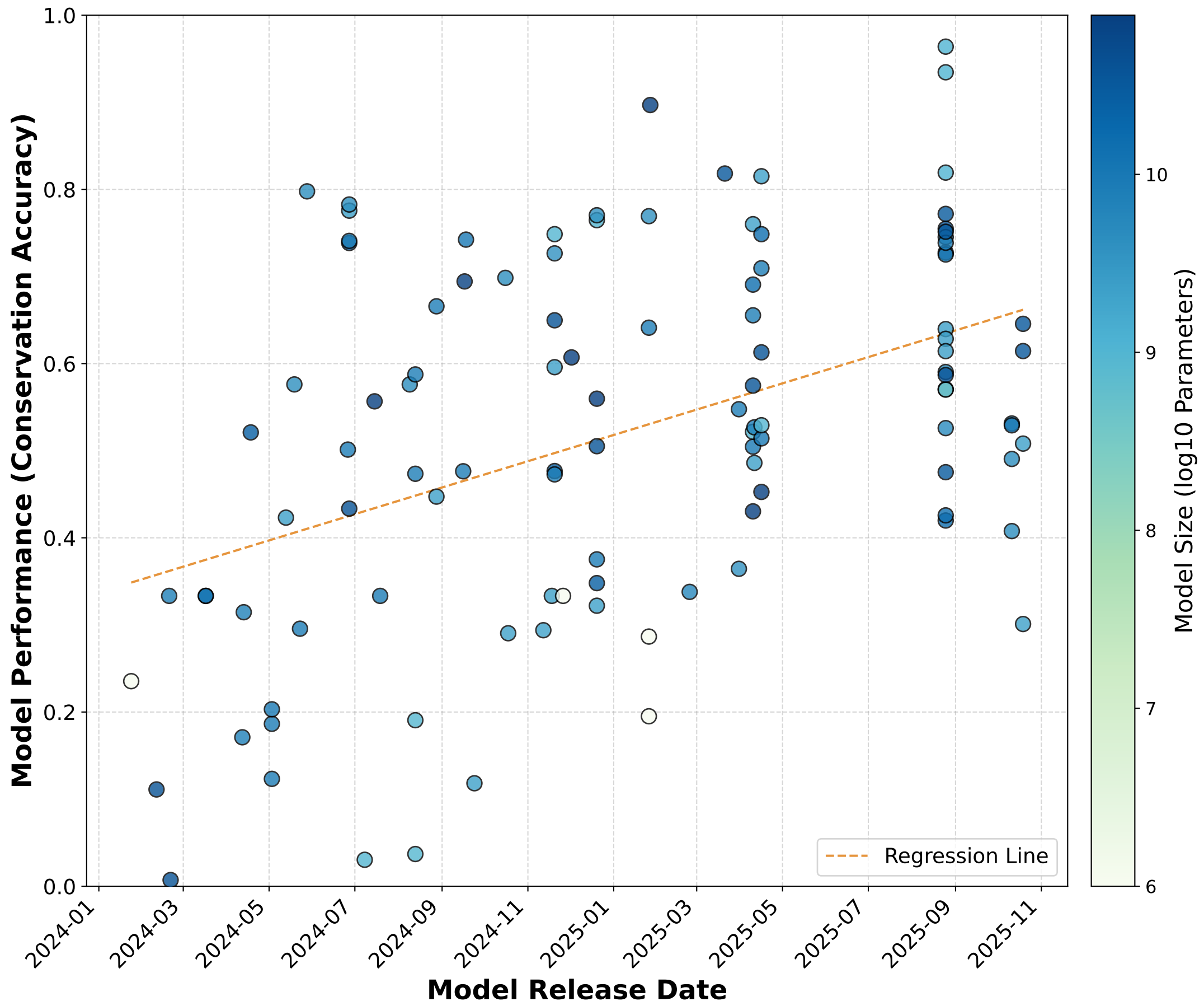
Model Performance (Conservation) vs Release Date
