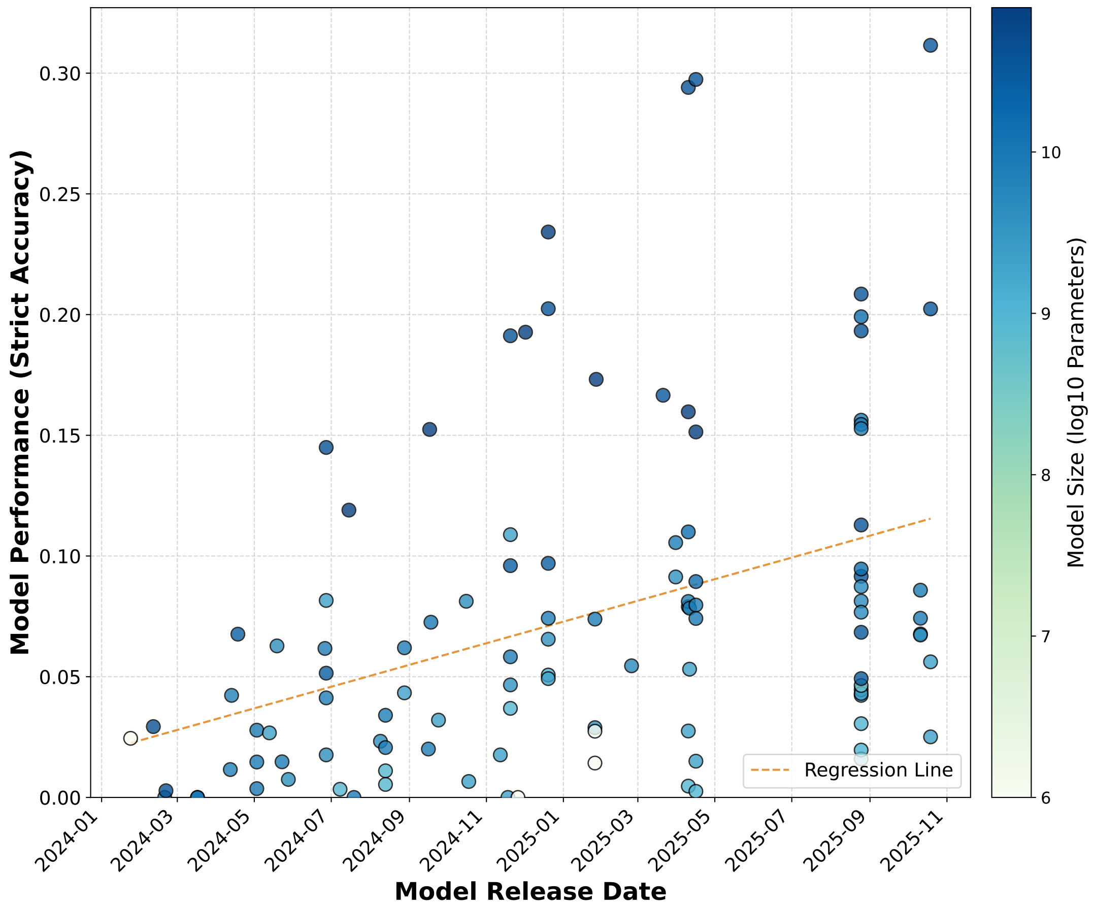
Model Performance (Strict) vs Release Date
