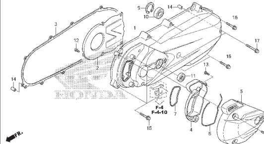
E-13 LEFT SIDE COVER
