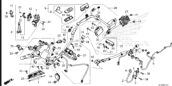
F-41-1 WIRE HARNESS/FOB KEY (WW150HV)
