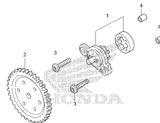
E-11 OIL PUMP
