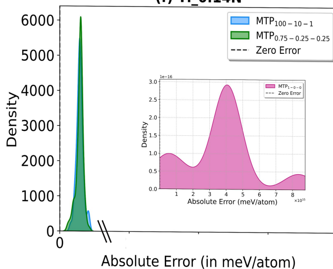
(f) Ti_{0.14}N
