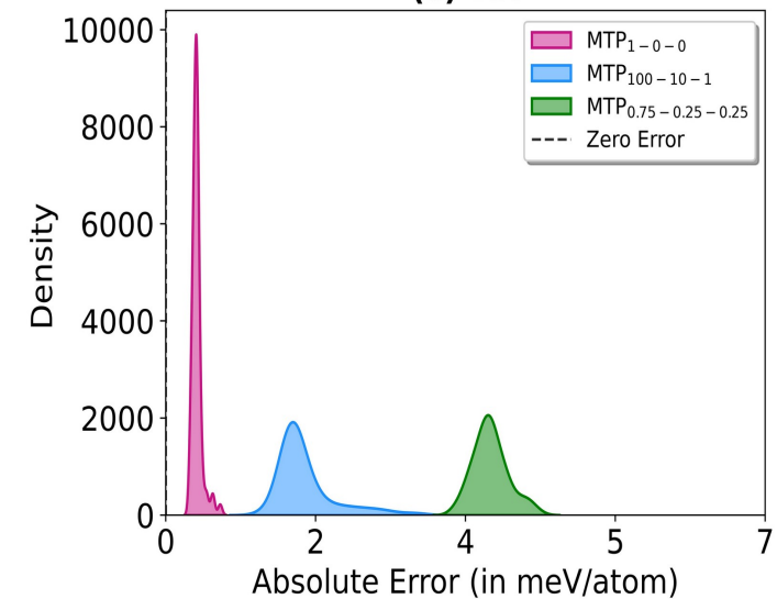
(e) TiN
