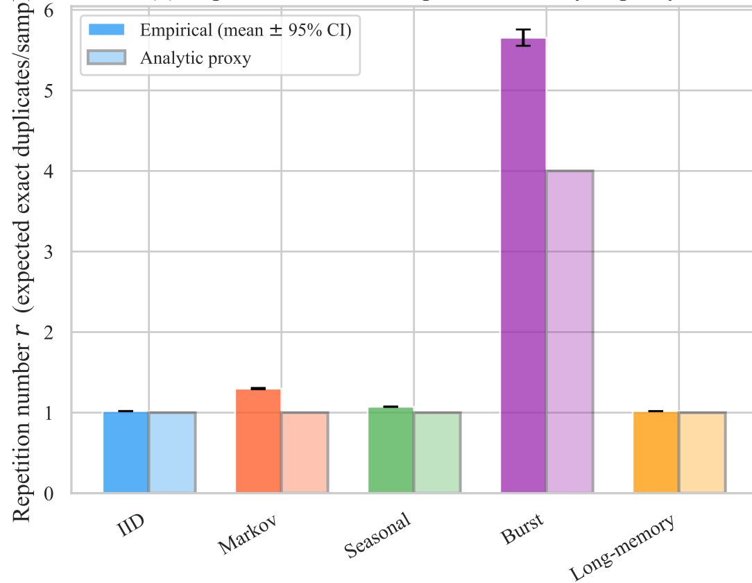
(b) Repetition number: empirical vs. analytic proxy
