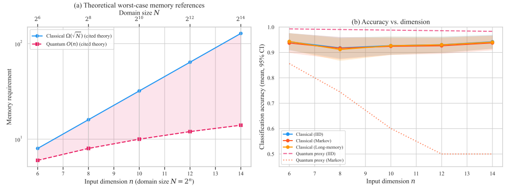
Figure 6. Dimension scaling analysis (10-seed-mean, 95% CI bands). (a) Worst-case Theoretical worst-case memory reference (cited bounds; no measured content): representative classical lower bound \Omega(\sqrt{N}) = \Omega(2^{n/2}) from the cited task-specific hardness results vs. quantum \mathcal{O}(n) . The gap separation is exponential in n at the level of theory; this is a worst-case reference, not a witnessed empirical floor for any classical baseline studied here (Section 3.3). (b) Classification accuracy vs. dimension n : classical online-SGD accuracy for IID, Markov, and long-memory data (solid lines; 10-seed mean, \pm 1.96 SE bands) compared with quantum-deterministic accuracy proxies for IID and Markov (dashed). The quantum-IID proxy is consistently near 1.0 (a task-level generalisation trend, not oracle-construction feasibility; Section 3.23.3); the quantum-analytic- \tau Markov proxy degrades with dimension (because \tau_{\text{Markov}} = n/(1-\rho) grows with n , reducing T_{\text{eff}} ), while classical accuracy is approximately stable across the range studied.
