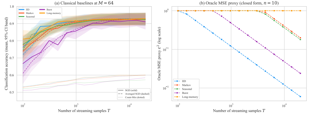
Figure 1. Classification accuracy and quantum-proxy error vs. stream length T (10-seed mean, 95% CI bands). (a) Three classical baselines at M = 64 (10-seed mean, \pm 1.96 SE bands): online SGD (solid), averaged SGD (dashed), Count-Min (dotted). (b) Quantum oracle MSE proxy \epsilon^2 (deterministic closed form, n = 10 qubits), log-log scale; no seed dependence.
