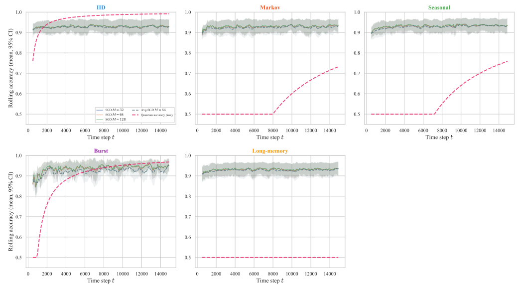
Figure 7. Rolling accuracy (window = 500) per regime; 10-seed mean \pm 95% CI. Classical SGD at M \in \{32, 64, 128\} (solid), averaged SGD M = 64 (dashed grey), quantum-accuracy proxy (dashed pink; analytic \tau ). Under IID and burst the proxy reaches or exceeds classical by horizon end; under Markov and seasonal it rises more slowly and remains below classical (conservative analytic \tau ); under long-memory the analytic- \tau proxy is pinned at 0.5 throughout ( the empirical- \tau placement of this regime differs; Section 6.9 ).
