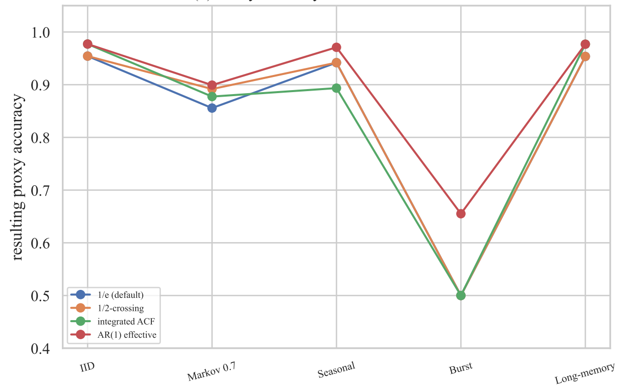
(b) Proxy accuracy under estimator choice
