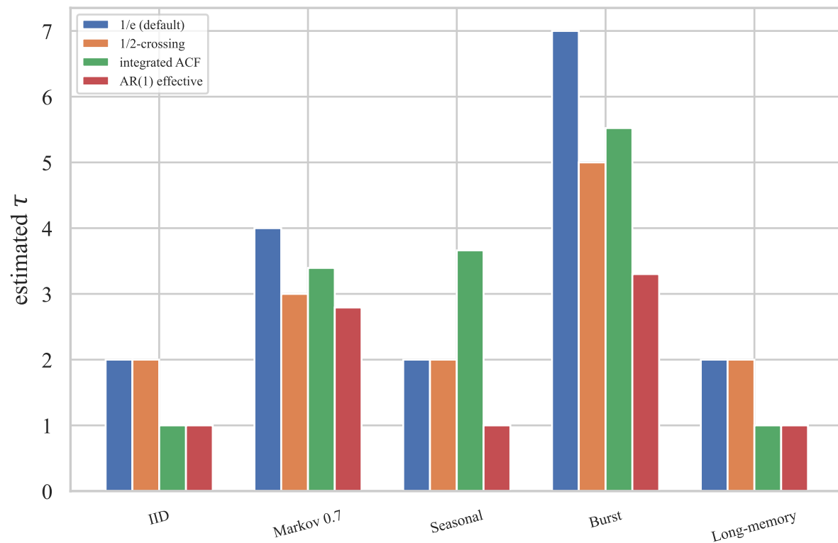
(a) Alternative \tau estimators on synthetic streams
