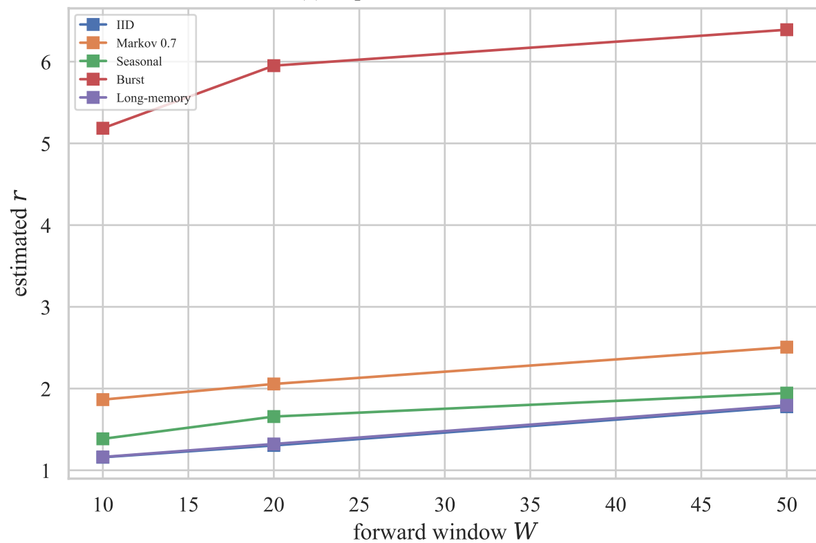
(c) Repetition r vs window size
