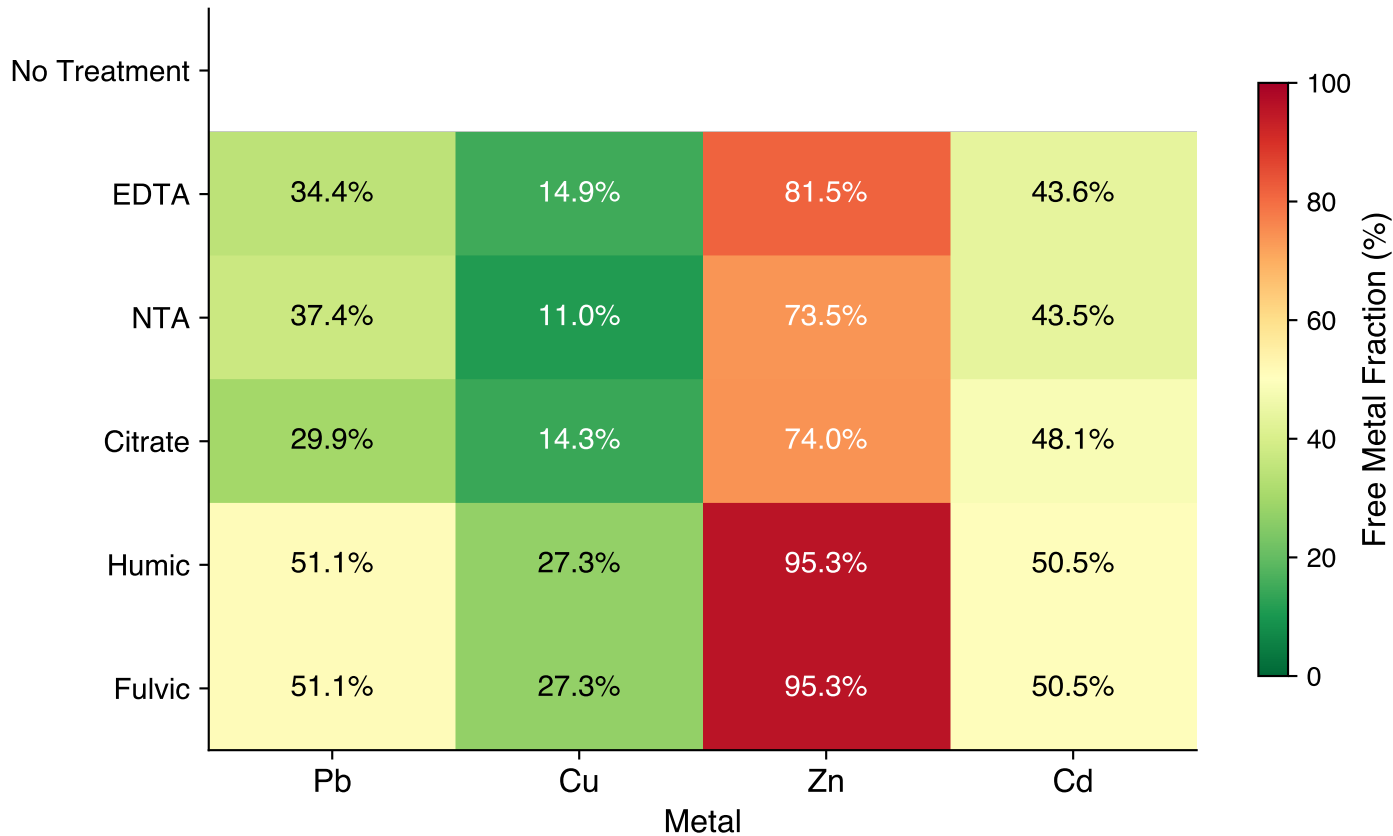
Mean Free Metal Fraction by Chelator at pH 7.0
