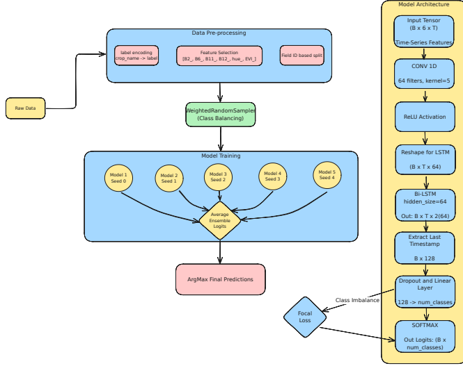
Fig. S5. Architecture of the CNN + BiLSTM model: 1D convolutional temporal feature extraction followed by a bidirectional LSTM.
