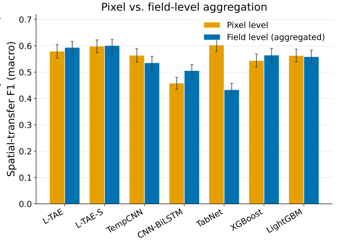
Fig. S9. Spatial-transfer macro-F1 at pixel versus field level. Field-level aggregation recovers transfer for dense temporal models (L-TAE, CNN-BiLSTM) but collapses the sparsity-reliant TabNet. Error bars are 95% bootstrap CIs over holdout fields.
