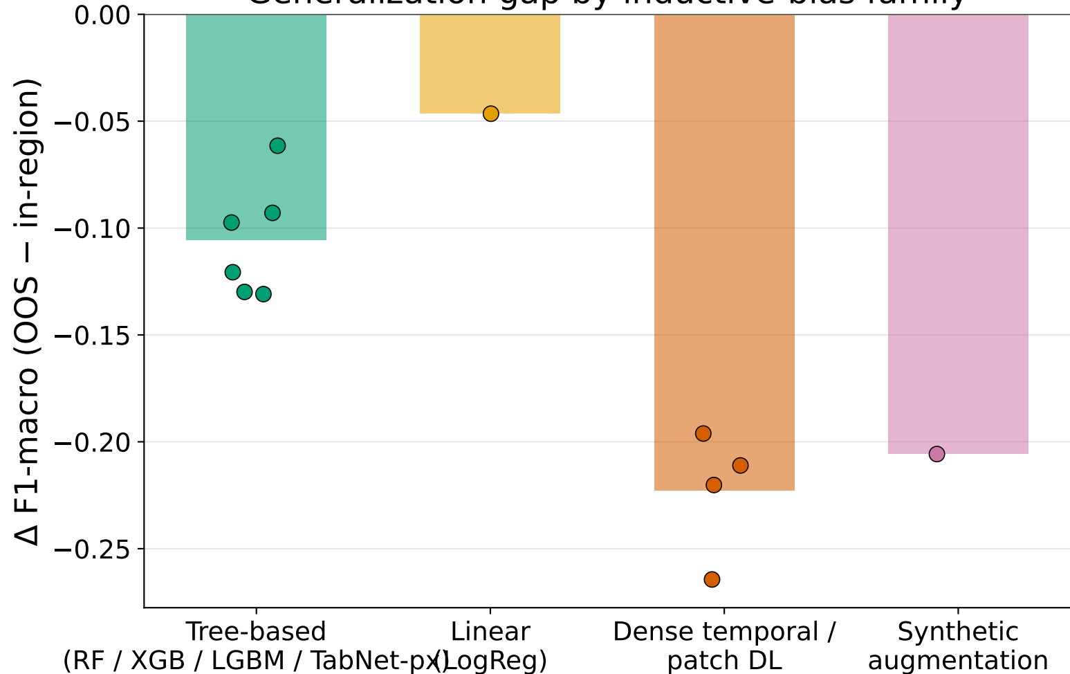
Generalization gap by inductive-bias family
