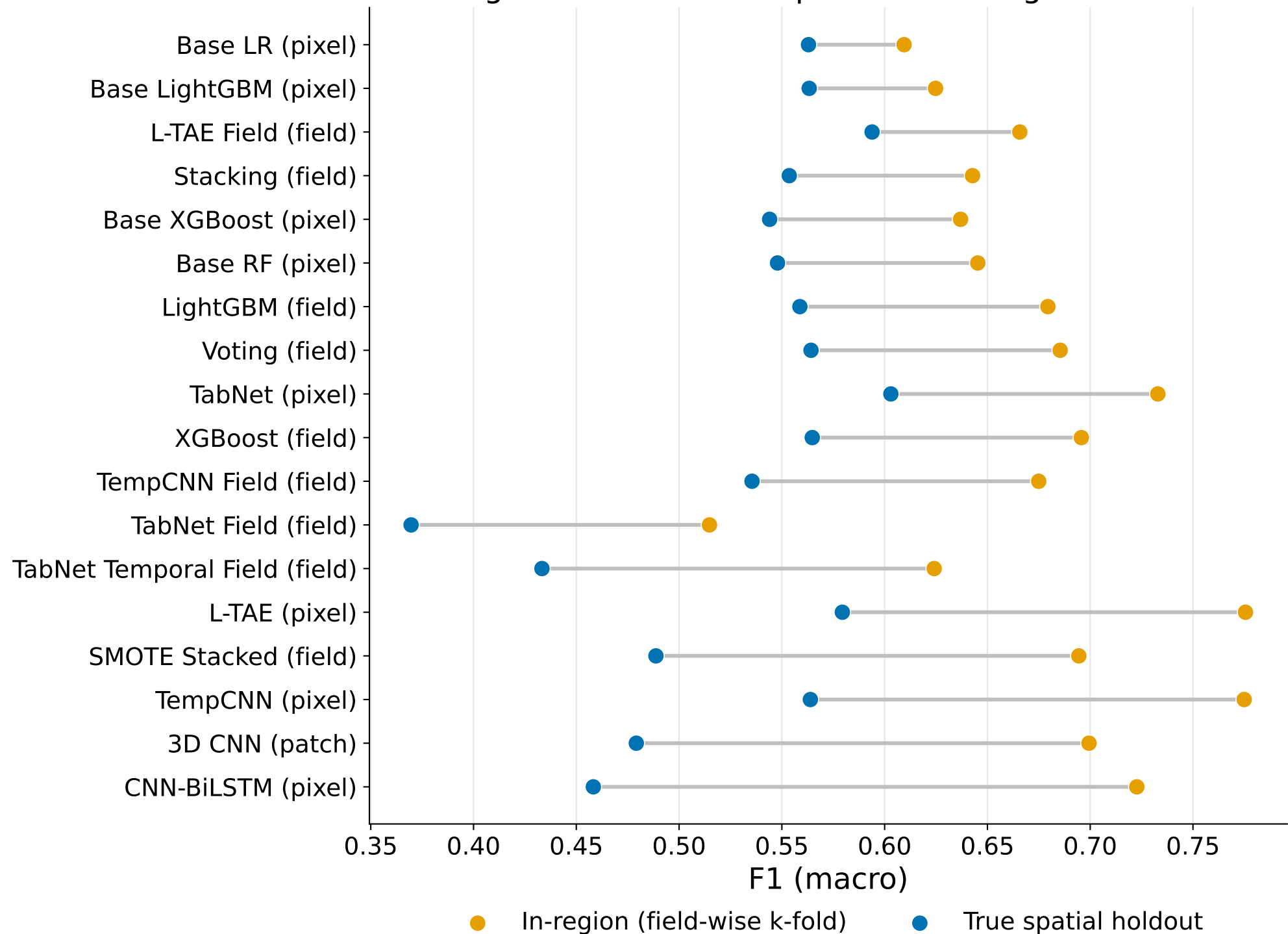
In-region validation vs. spatial-holdout generalization
