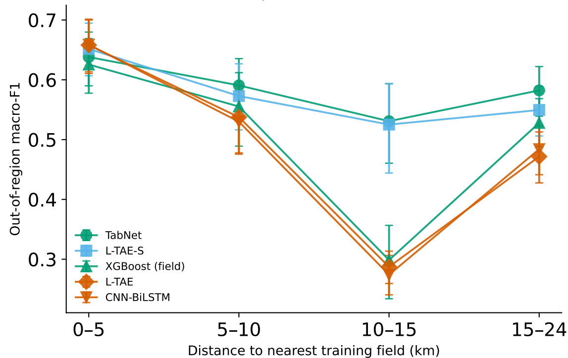
(a) Representative models
