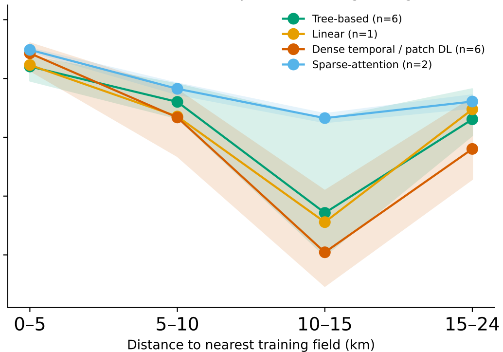
(b) Inductive-bias family mean (shading = range)
