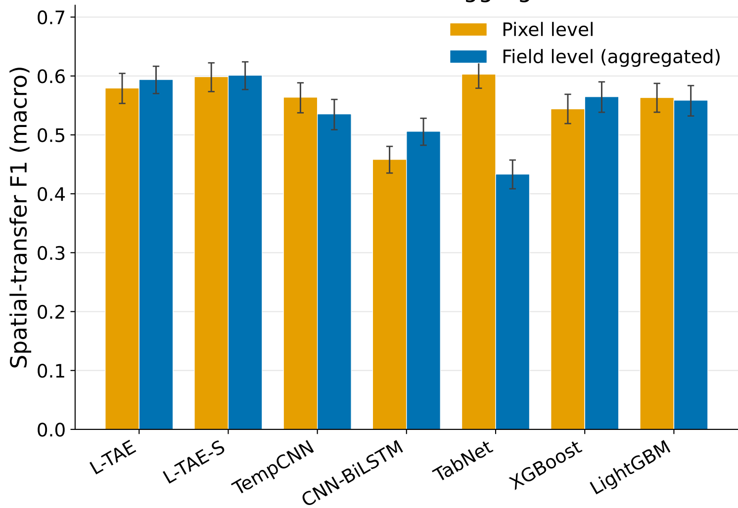
Pixel vs. field-level aggregation
