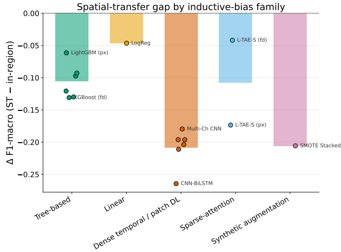
Fig. 3. Spatial-transfer gap ( \Delta macro-F1) grouped by inductive-bias family. Sparse/tree-like and linear models transfer (small |\Delta| ); dense temporal/patch nets and synthetic augmentation overfit the training region. L-TAE-S, which adds sparse feature selection to a dense attention backbone, tracks the tree-based models. Bars are family means; points are individual models.
