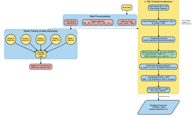
Fig. 1. Architecture of the sparse-attention L-TAE-S. Before the multi-head temporal attention, a TabNet-style sparse feature gate (highlighted) applies a per-head sparsemax mask that selects a small subset of embedding channels, with a relaxation prior ( \gamma = 1.5 ) discouraging heads from re-selecting the same channels. This block is the only architectural difference from the L-TAE; five seeds are ensembled and aggregated to field level.
