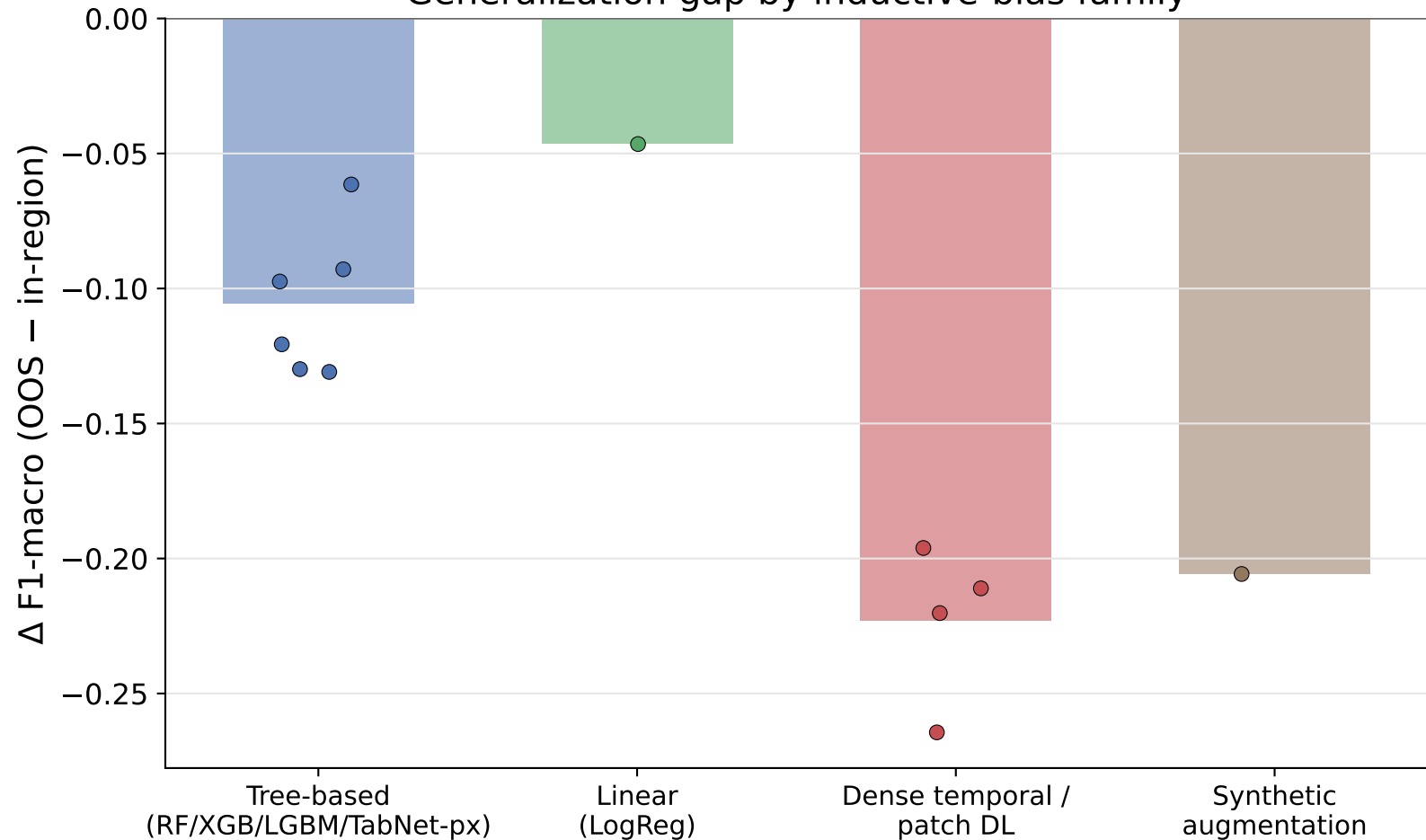
Generalization gap by inductive-bias family
