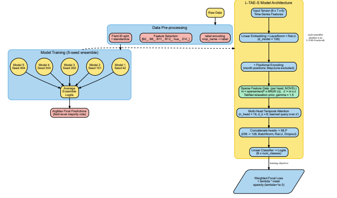
Fig. 1. Architecture of the sparse-attention L-TAE-S. Before the multi-head temporal attention, a TabNet-style sparse feature gate (highlighted) applies a per-head sparsemax mask that selects a small subset of embedding channels, with a relaxation prior ( \gamma = 1.5 ) discouraging heads from re-selecting the same channels. This block is the only architectural difference from the L-TAE; five seeds are ensembled and aggregated to field level.
