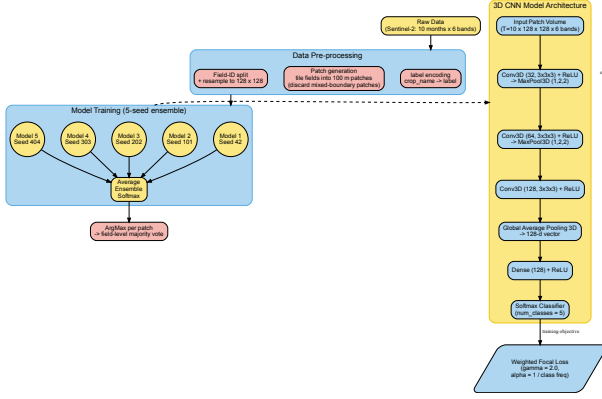
Fig. S9. Patch-level 3D CNN pipeline: each field is tiled into 100 m patches resampled to 128 \times 128 ; a five-seed ensemble averages softmax outputs, and per-patch predictions are aggregated to a field label by majority vote.
