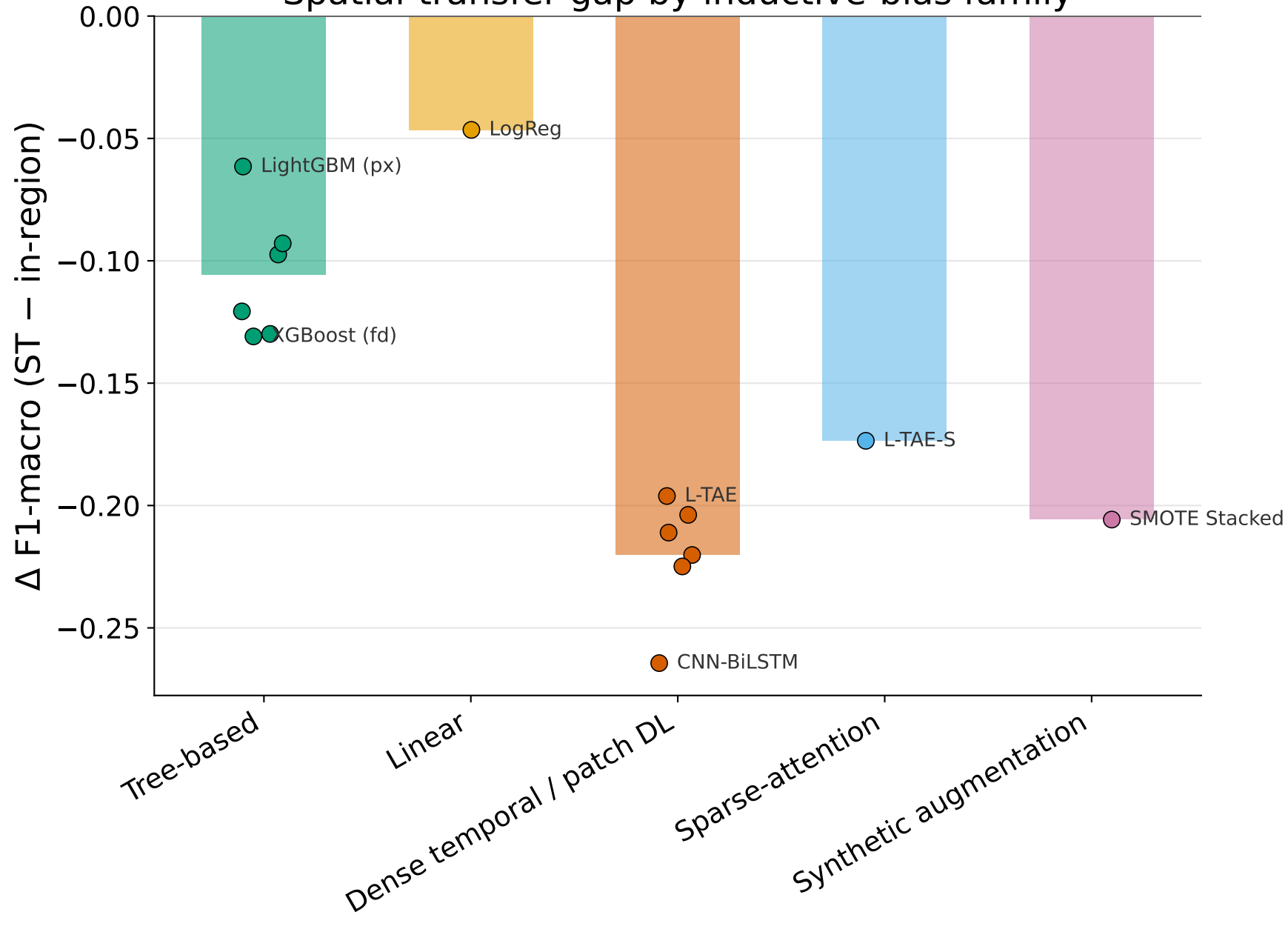
Spatial-transfer gap by inductive-bias family
