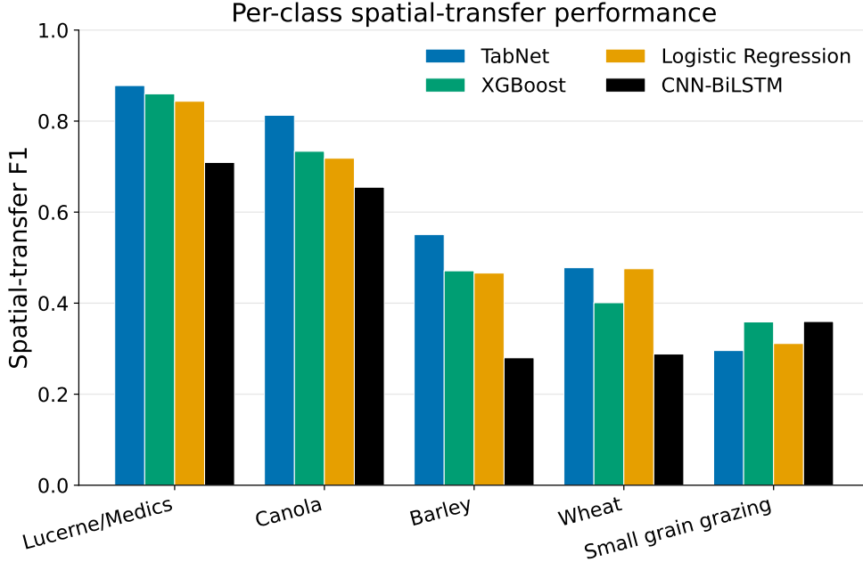
Fig. 14: Per-class spatial-transfer F1 for four representative models.
