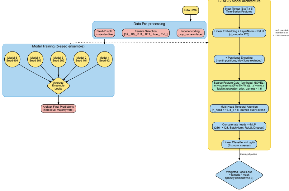
Fig. 8: Architecture of the sparse-attention L-TAE-S.
