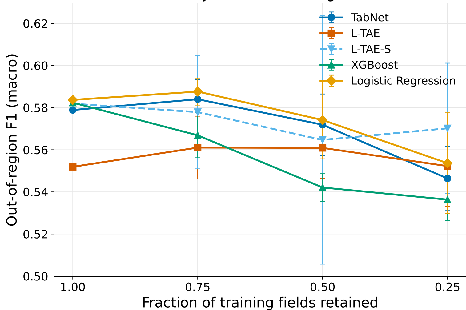
Data efficiency under out-of-region transfer
