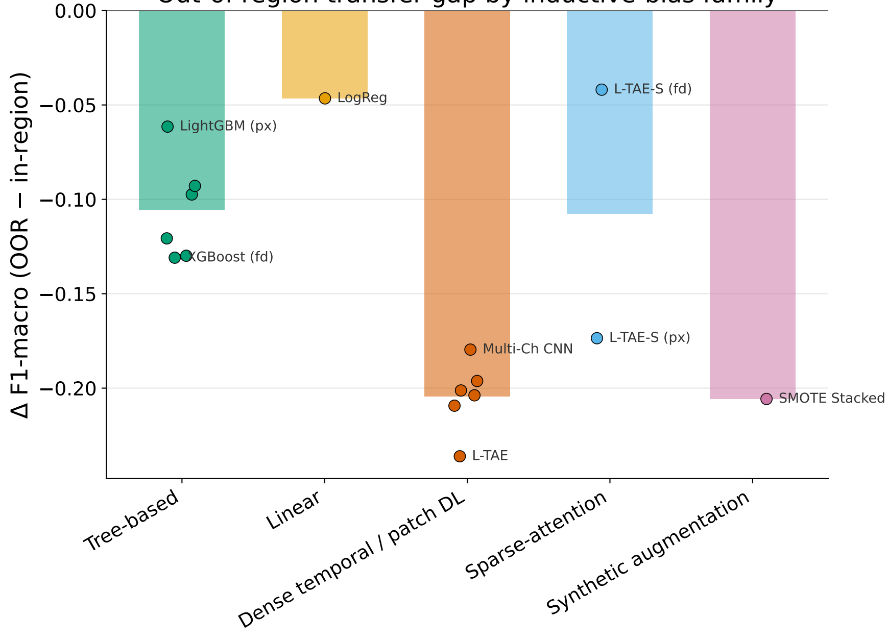
Out-of-region transfer gap by inductive-bias family
