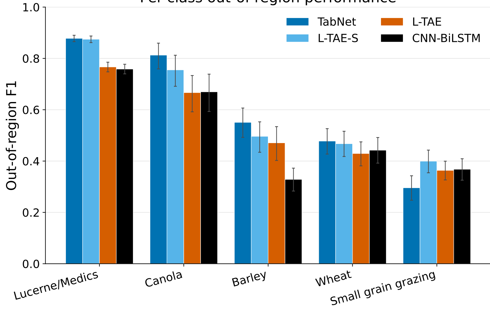
Per-class out-of-region performance
