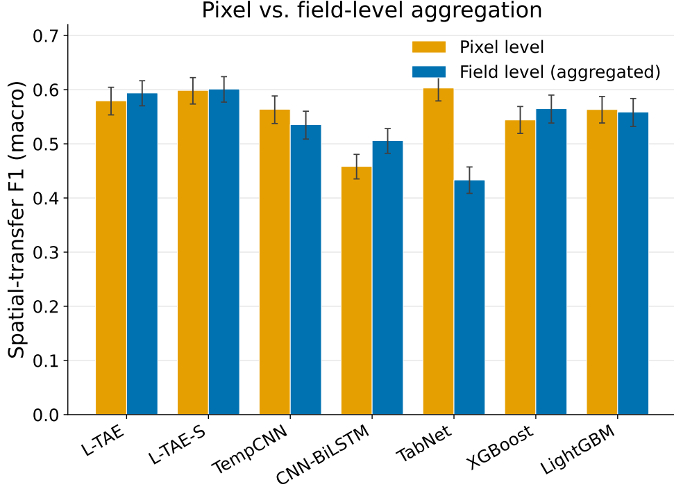
Fig. 12: Spatial-transfer F1_m at pixel versus field level.
