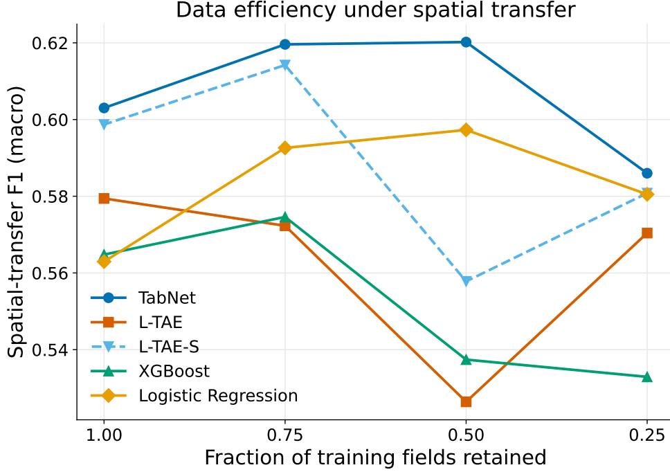
Fig. 13: Spatial-transfer F1 m versus fraction of training fields.
