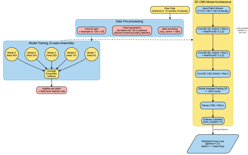
Fig. 10: Patch-level 3D CNN pipeline. Each field is tiled into 100m patches and resampled to 128 \times 128 ; a single multiclass 3D CNN is trained as a five-seed ensemble whose softmax outputs are averaged, and per-patch predictions are aggregated to a field label by majority vote.
