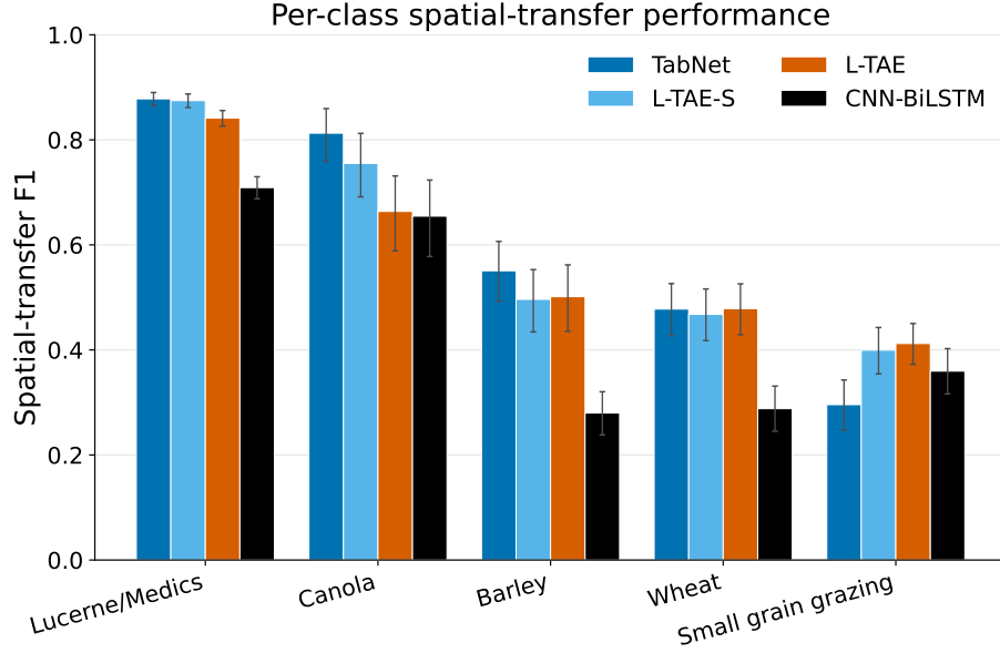
Figure 3: Per-class F1 on the holdout region for four representative models (TabNet, L-TAE-S, L-TAE, and CNN-BiLSTM). TabNet, L-TAE-S, and L-TAE classify lucerne/medics and canola well; the cereals (barley, wheat) and small-grain grazing concentrate the errors. CNN-BiLSTM’s accuracy drops on every class. Error bars are 95% bootstrap CIs over holdout fields.
