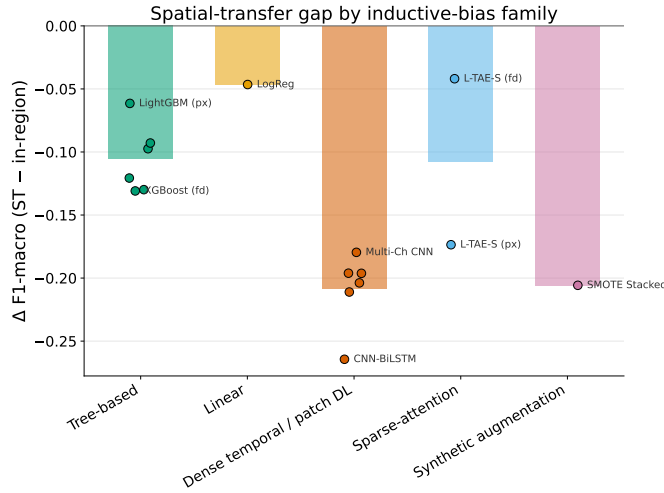
Fig. 5. Spatial-transfer gap ( \Delta macro-F1) grouped by inductive-bias family. Sparse/tree-like and linear models transfer (small |\Delta| ); dense temporal/patch nets and synthetic augmentation overfit the training region. L-TAE-S, which adds sparse feature selection to a dense attention backbone, tracks the tree-based models. Bars are family means; points are individual models.
