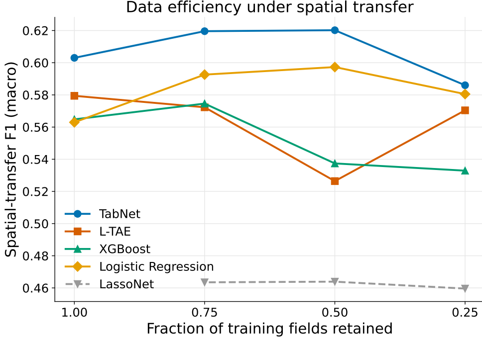
Fig. 14: Spatial-transfer macro-F1 as the number of training fields is reduced to 75%, 50%, and 25%. Robust models (TabNet, logistic regression) are nearly flat; LassoNet is weak throughout.
