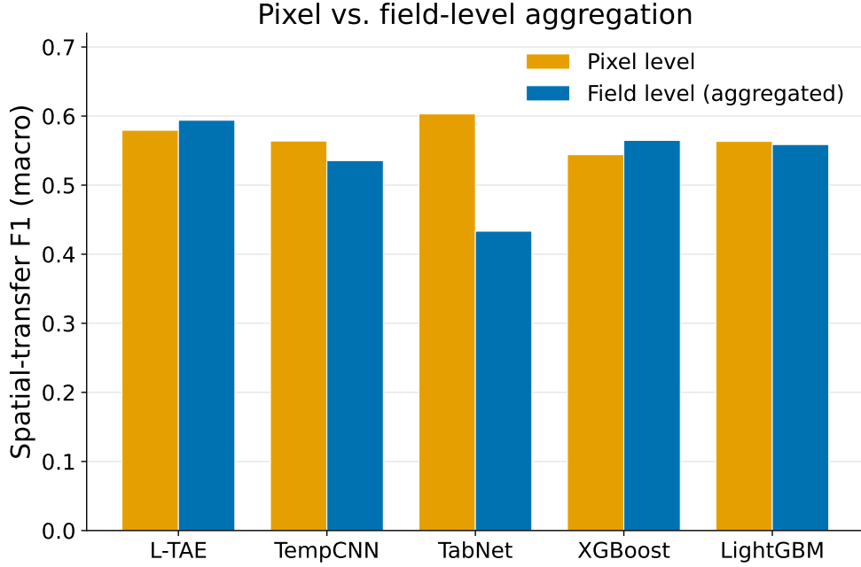
Fig. 13: Spatial-transfer macro-F1 at pixel versus field level. Field-level aggregation recovers transfer for dense temporal models (L-TAE) but collapses the sparsity-reliant TabNet.
