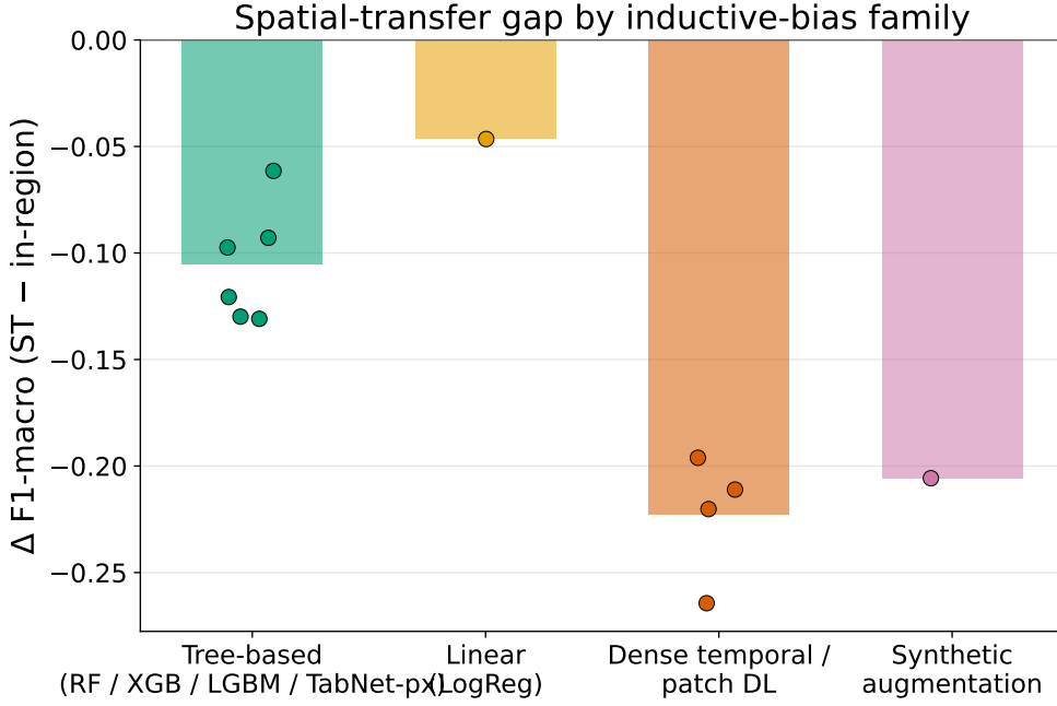
Fig. 16: Generalization gap ( \Delta macro-F1, spatial-transfer minus in-region) grouped by inductive-bias family. Sparse/tree-like and linear models transfer (small |\Delta| ); dense temporal/patch deep nets and synthetic augmentation overfit the training region. Bars show family means; points are individual models.
