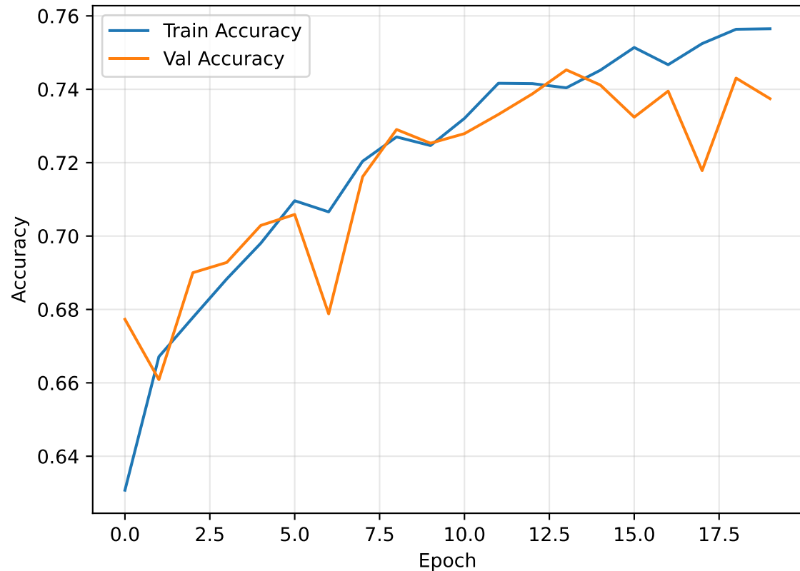
Training Accuracy
