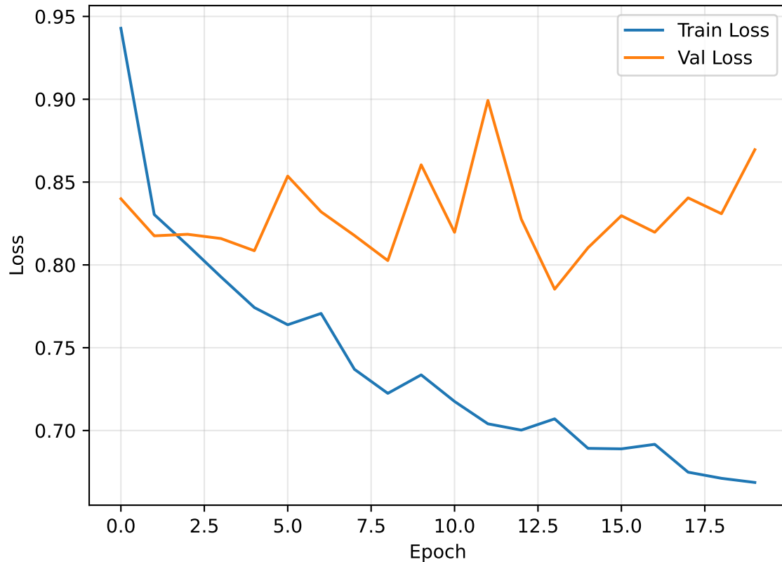
Training Loss
