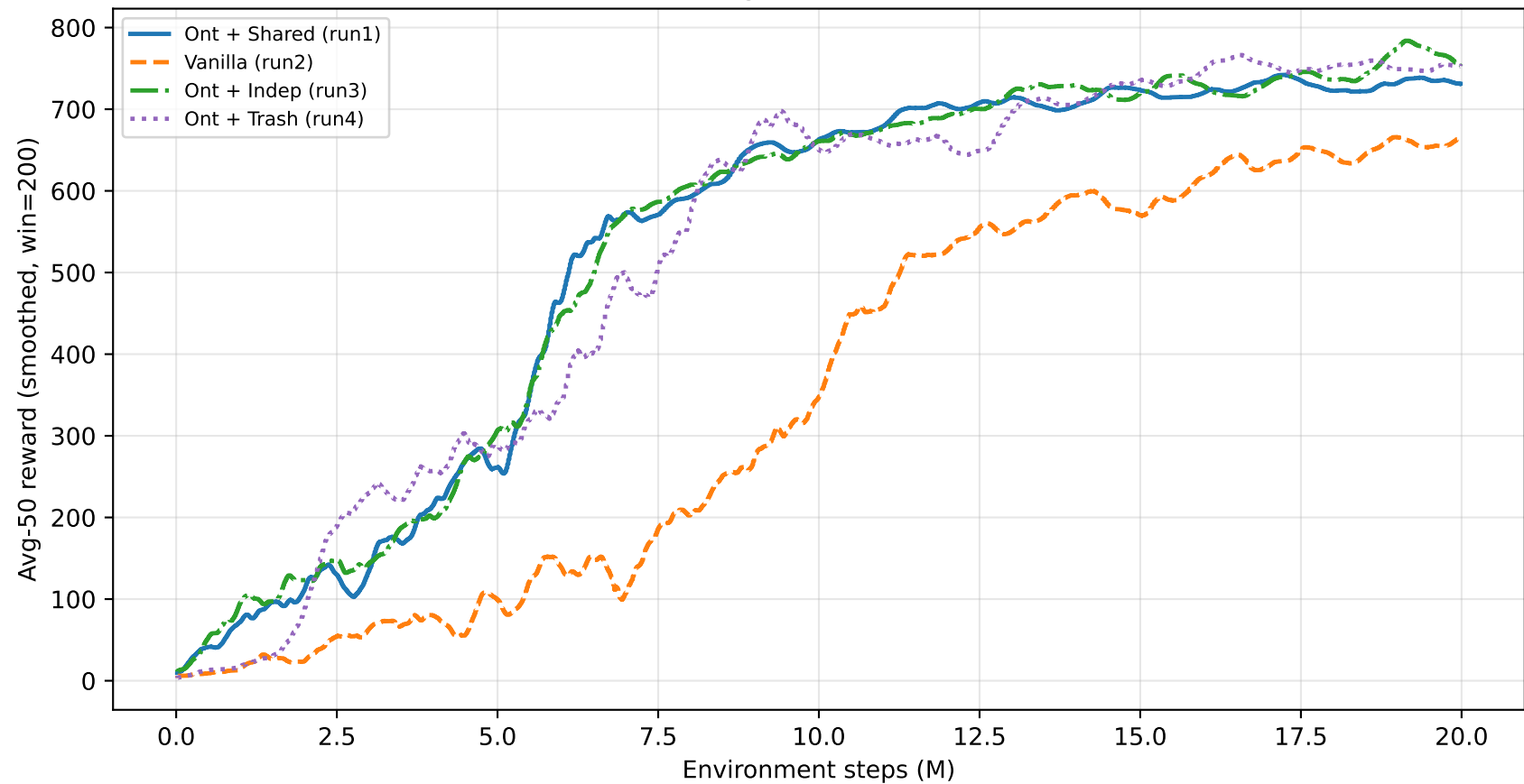
Training reward: all runs
