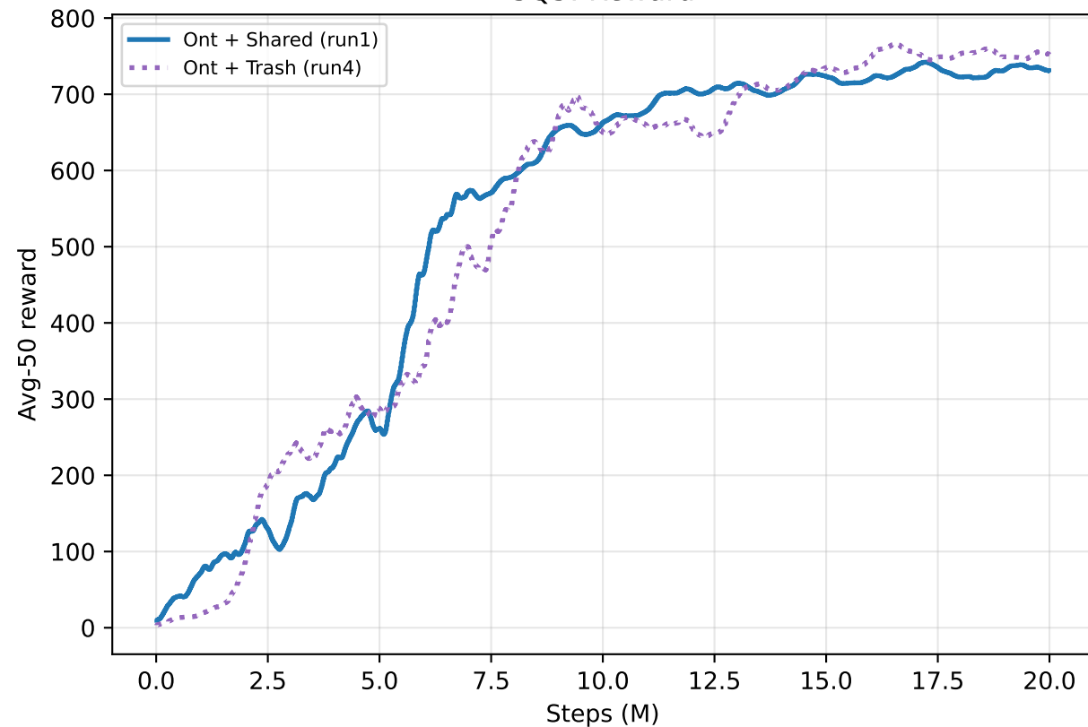
SQ5: Reward
