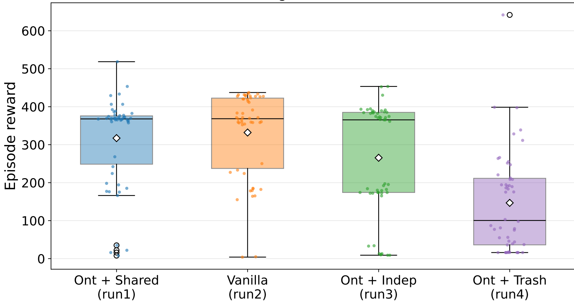
Evaluation reward over 50 stochastic episodes (Stage 2, 4 items)
