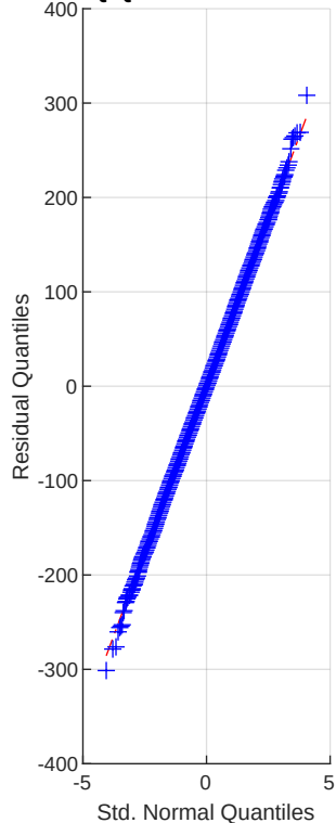
Q-Q Plot of Residuals
