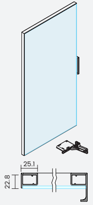
LB.SF.2Q.04 隐框天地铰链玻璃门 ( 轻型 ) LB.SF.2Q.04 Hidden Frame Heaven Earth Hinged Glass Door (Lightweight)
