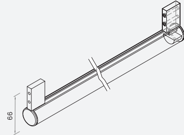
衣通 3 代侧装 (层板离地 >1600 选用) 3rd Gen Side-Mount Hanging Rail (Use when shelf height from floor > 1600mm)
