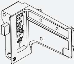
H7 吊码 深度 D>350mm 用于冰箱吊柜 H7 hanging code D> 350mm for refrigerator hanging cabinet
