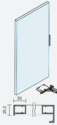
LB.SF.2Z.02 方形天地铰链玻璃门 ( 重型 ) LB.SF.2Z.02 Square Heaven Earth Hinged Glass Door (Heavy Duty)
