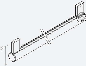
衣通 3 代顶装 (层板离地 >1600 选用) 3rd Gen Top-Mount Hanging Rail (Use when shelf height from floor > 1600mm)
