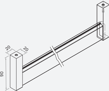
衣通 2 代顶装 (层板离地 >1600 选用) 2nd Gen Top-Mount Hanging Rail (Use when shelf height from floor > 1600mm)
