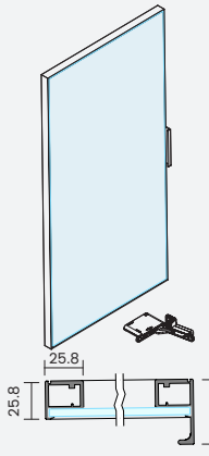
LB.SF.2Q.03 方形天地铰链玻璃门 ( 轻型 ) LB.SF.2Q.03 Square Heaven Earth Hinged Glass Door (Lightweight)
