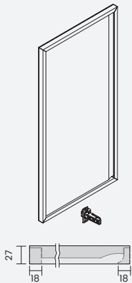
MLS.G4.0.10 四边骨骼线门 Mls.g4.0.10 Four-Sided Skeleton Door
