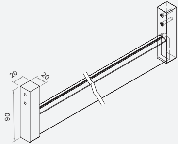
衣通 2 代侧装 (层板离地 >1600 选用) 2nd Gen Side-Mount Hanging Rail (Select when shelf height above floor > 1600mm)
