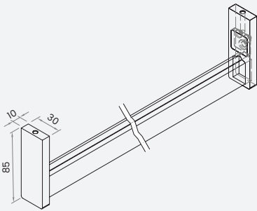
衣通 (顶装 / 侧装通用) Hanging Rail (Top/Side Mount)
