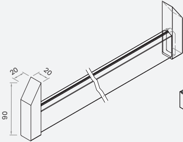
斜边衣通 (搭配斜边铝框层板用) Slanted Hanging Rail (For Slanted Aluminum Frame Shelf)
