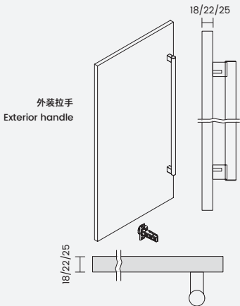
MLS.W1.0.13 双孔长拉手 Mls.w1.0.13 Double-Hole Long Handle
