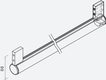
衣通 3 代顶装 (层板离地 >1600 选用) 3rd Gen Side-Mount Hanging Rail (Use when shelf height from floor > 1600mm)
