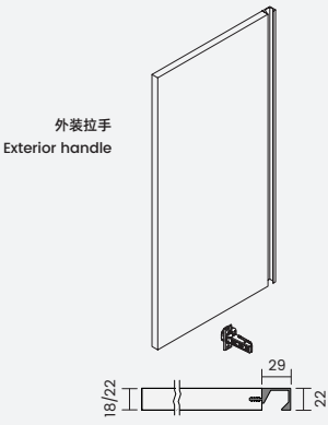
MLS.G.0.12 G 拉手 Mls.f.0.12 G Pull Handle Door
