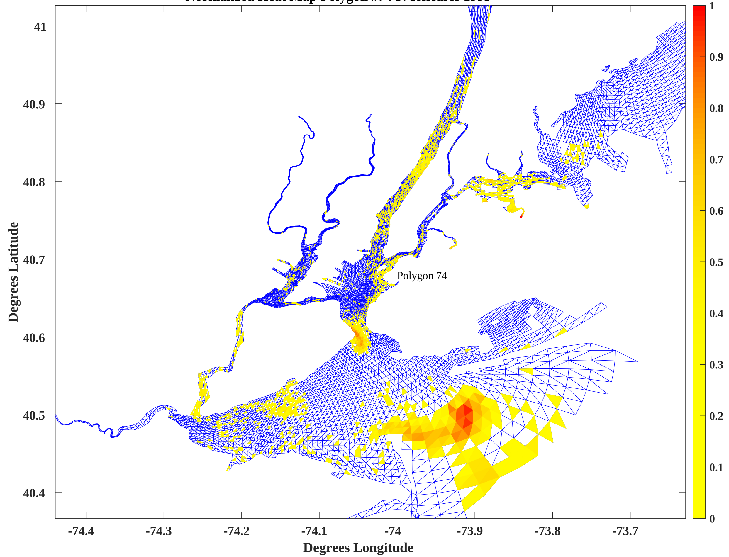
Normalized Heat Map Polygon #74 5: Releases 1993
