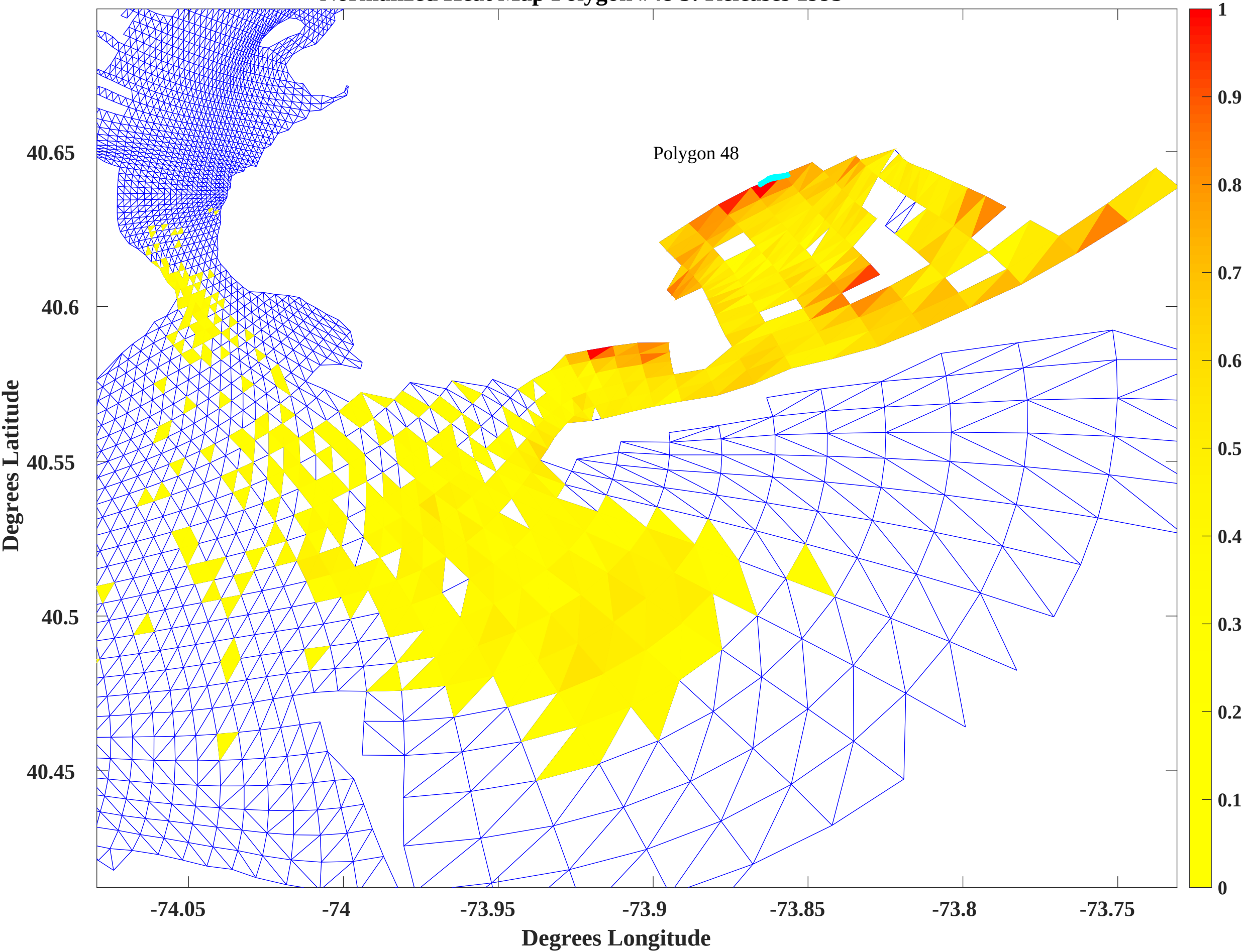
Normalized Heat Map Polygon #48 5: Releases 1995
