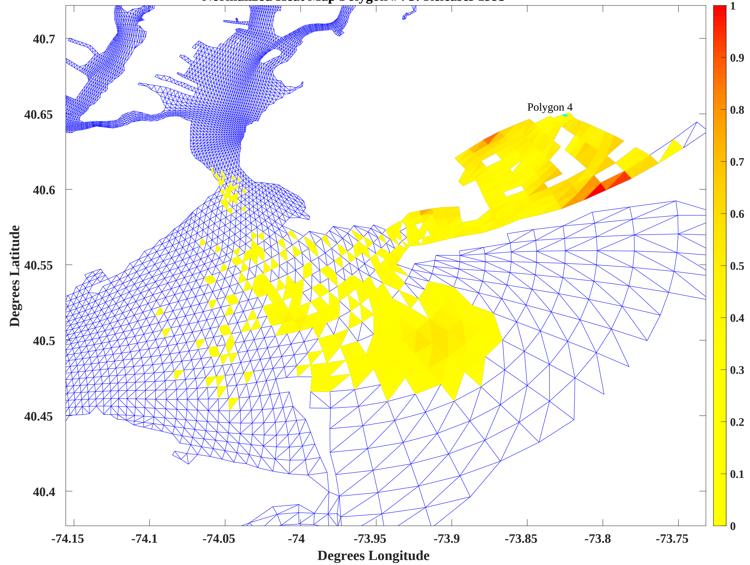
Normalized Heat Map Polygon #4 5: Releases 1993
