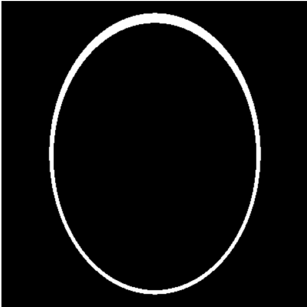
Soft Tissue Window C=40, W=400
