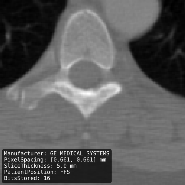
CT Image (raw)
