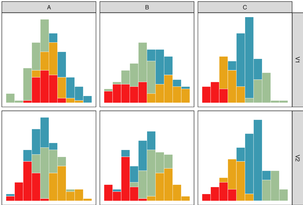
Figure 2: The typical approach to understanding the data partitions is plotting individual features using histograms, where group is mapped to colour. Here, the three data sets displayed in Figure 1 are shown in the columns, and the rows correspond to the two variables, V1, V2. Differences between groups can be seen, and interpreted on a single variable level, such as the red group has low values on both V1 and V2 in data set C. But how the data is divided cannot be seen.
