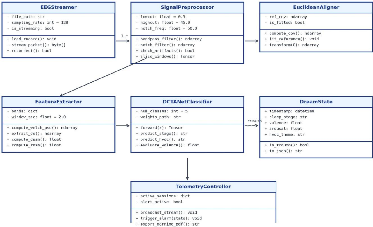
UML Class Diagram: Dreams2Reality Architecture
