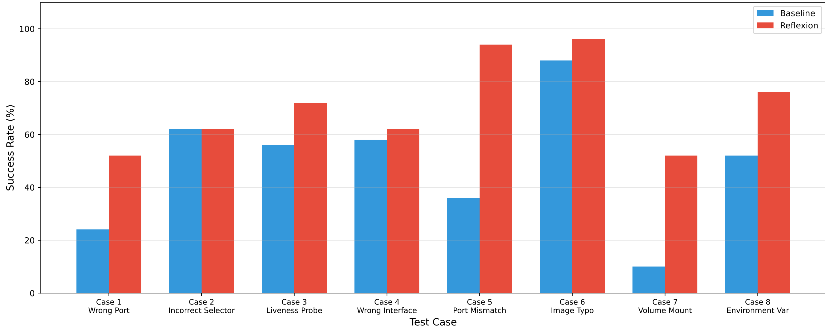
Success Rate by Test Case: Baseline vs Reflexion
