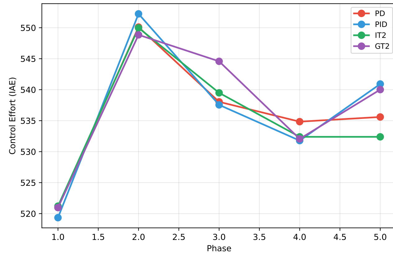
Control Effort Across Phases
