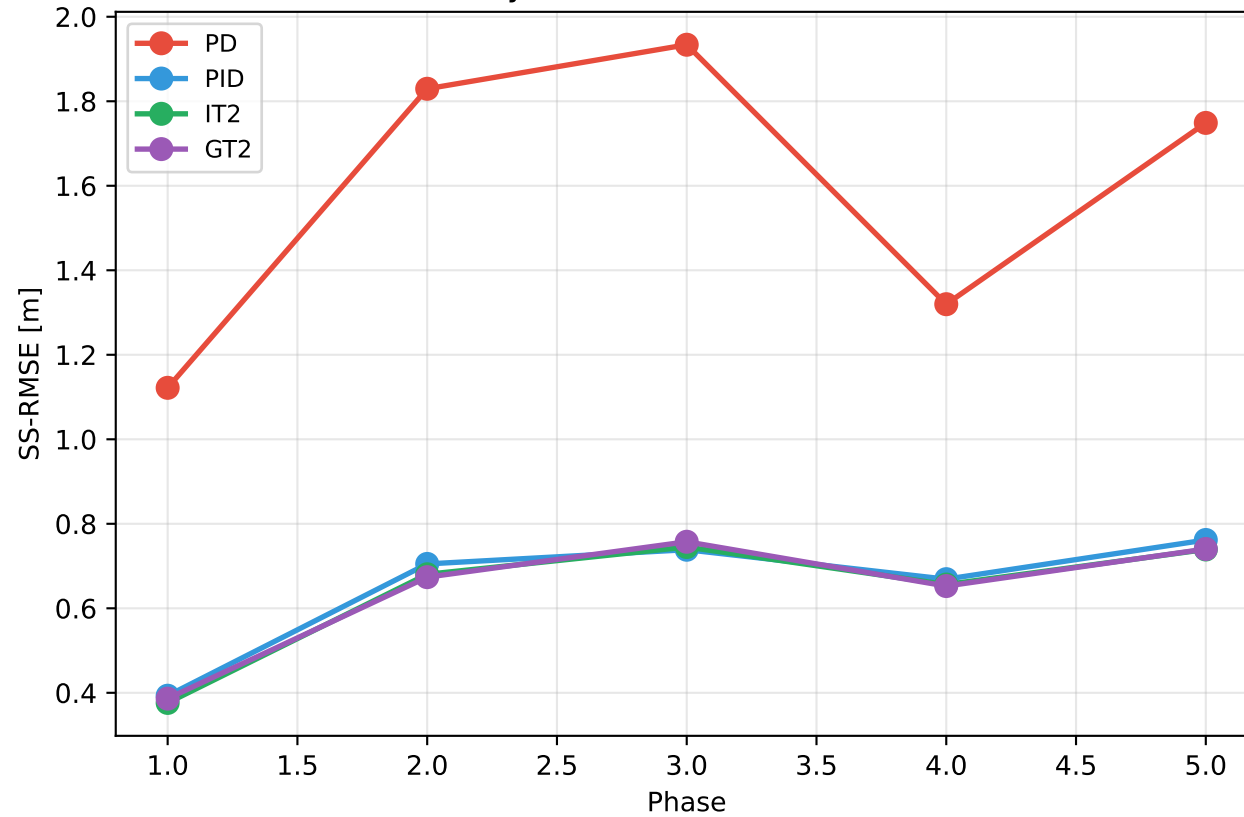
Steady-State RMSE Across Phases
