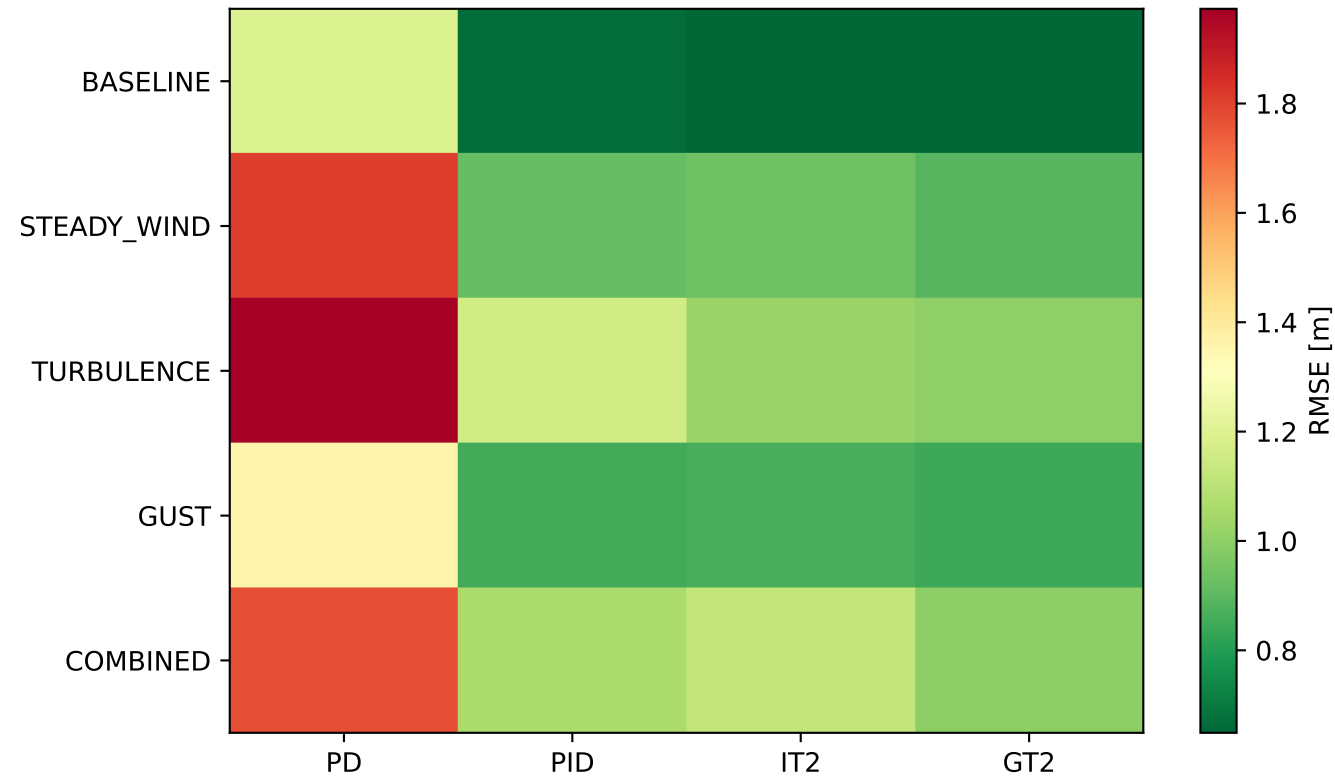
RMSE Heatmap (Phase × Controller)
