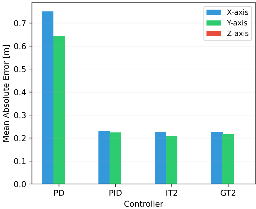
XYZ Error Decomposition - Phase 1
