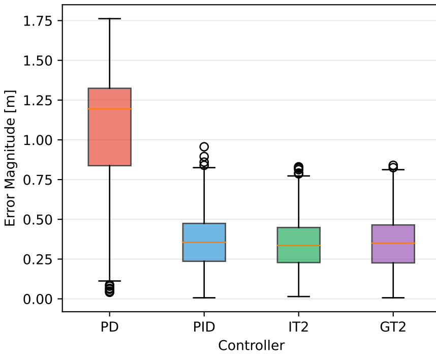
Steady-State Error Distribution - Phase 1
