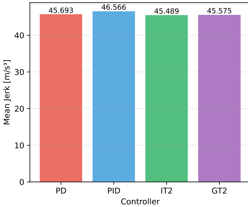
Jerk Analysis (Smoothness) - Phase 1
