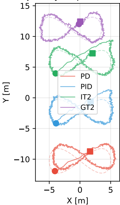
2D Trajectory (Top View) - Phase 1
