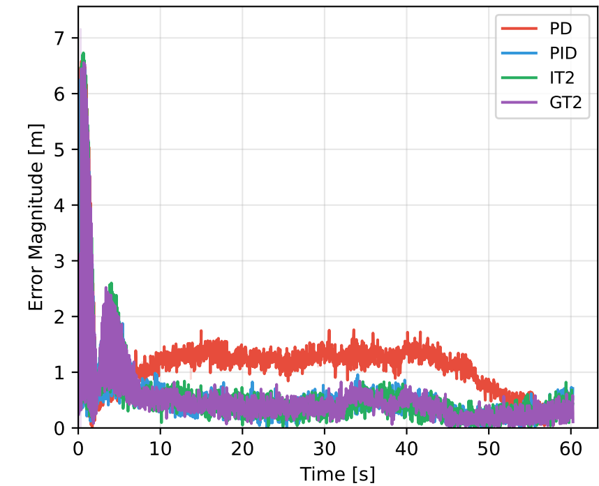
RMSE Evolution - Phase 1 (BASELINE)
