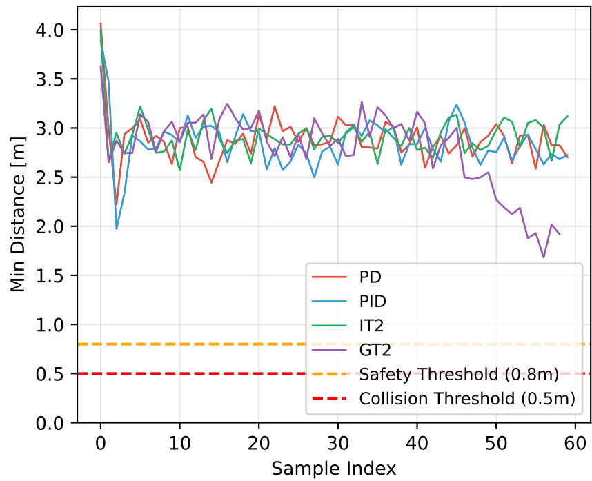
Min Inter-Agent Distance - Phase 1
